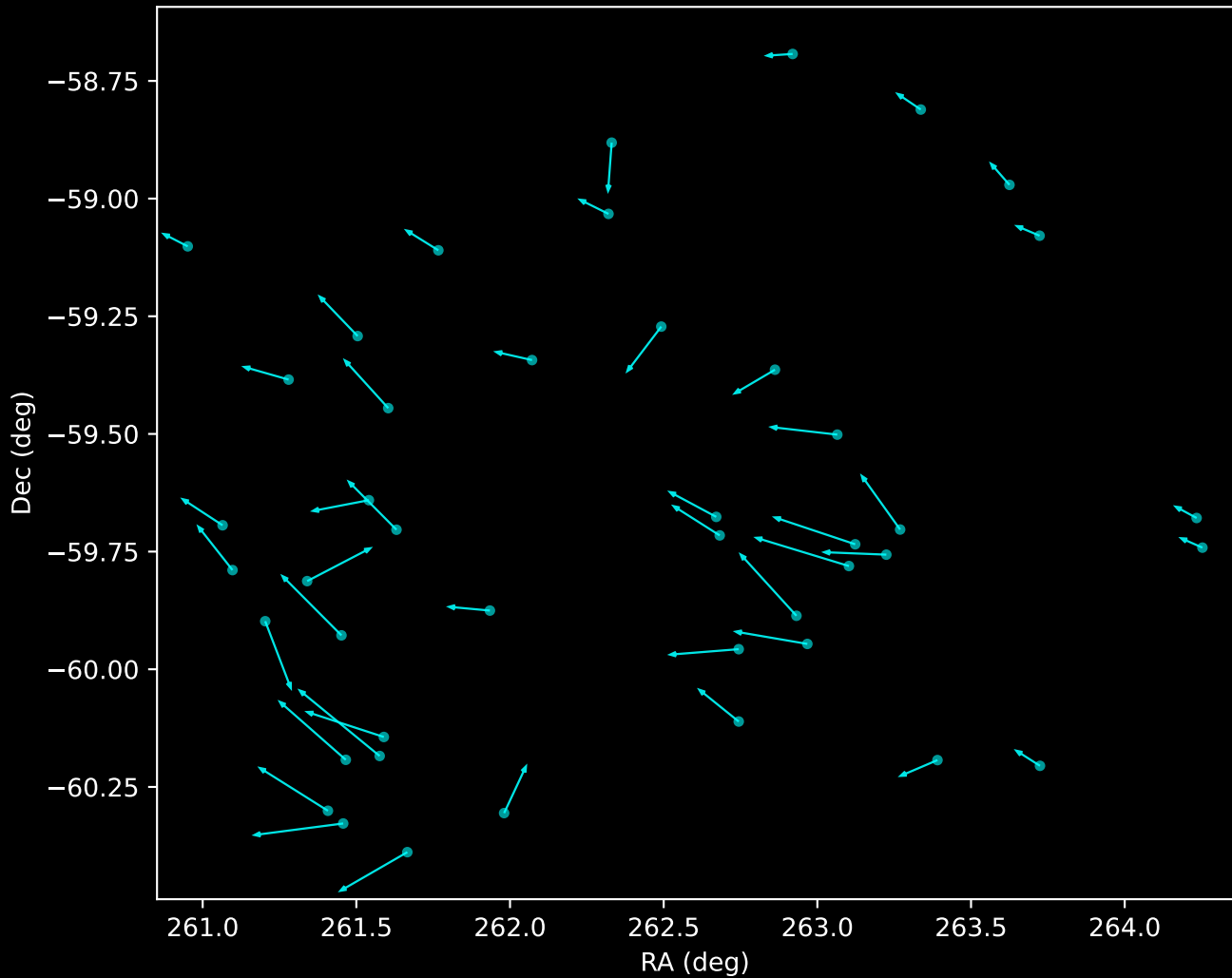
APOGEE DR17 Noise Stream Proper Motion Vectors (n=44)
