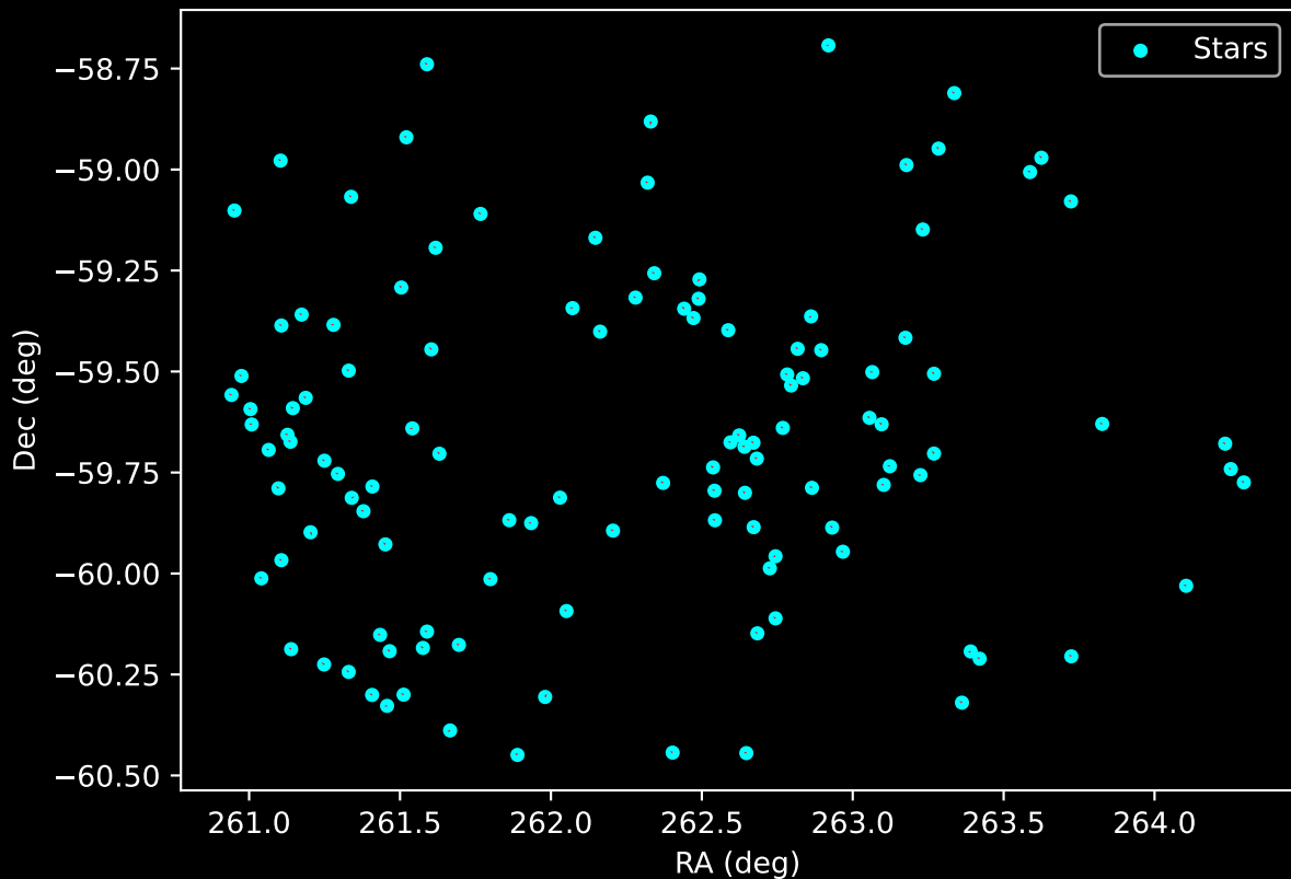
APOGEE DR17 Field: [288-00-C] Proper Motion Vectors for Gaia Star Field (n= 119)
