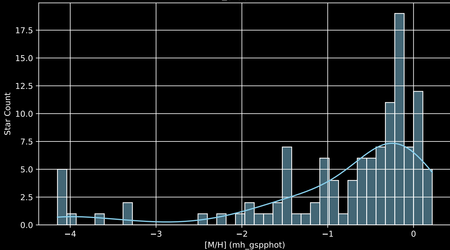
APOGEE DR17 Field: [288-00-C [M/H] (mh_gspphot) (n= 117)
