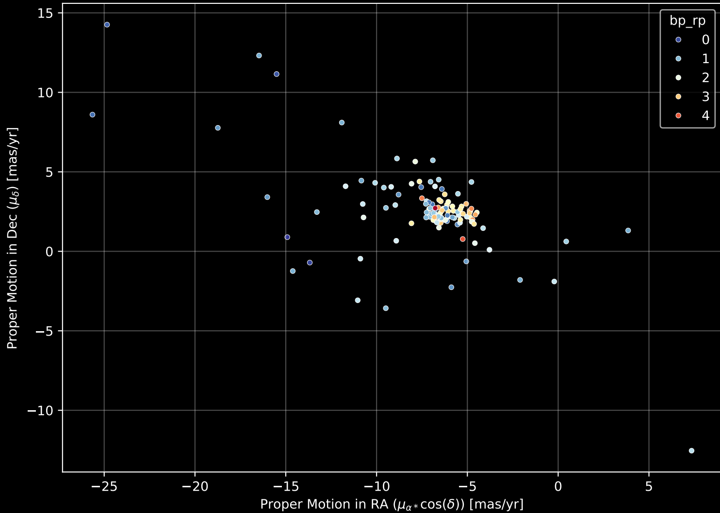
APOGEE DR17 Field: [288-00-C] Proper Motion Diagram (n= 119)
