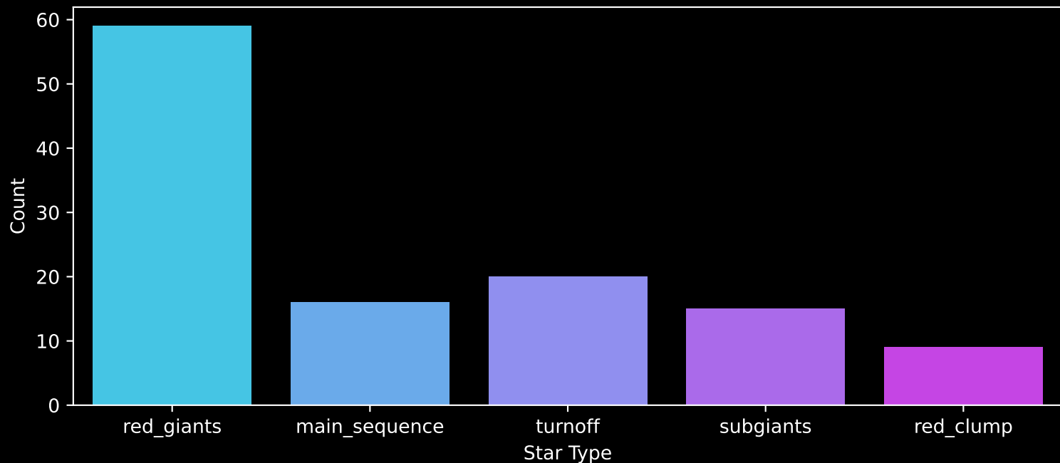
APOGEE DR17 Field: [288-00-C] Count plot of Star Type
