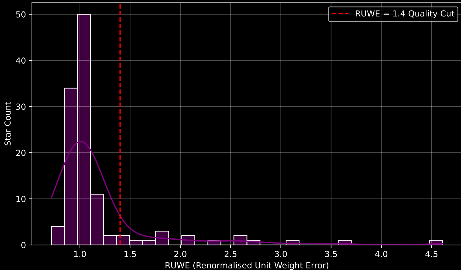
GAPOGEE DR17 Field [288-00-C] RUWE Distribution (n= 117)
