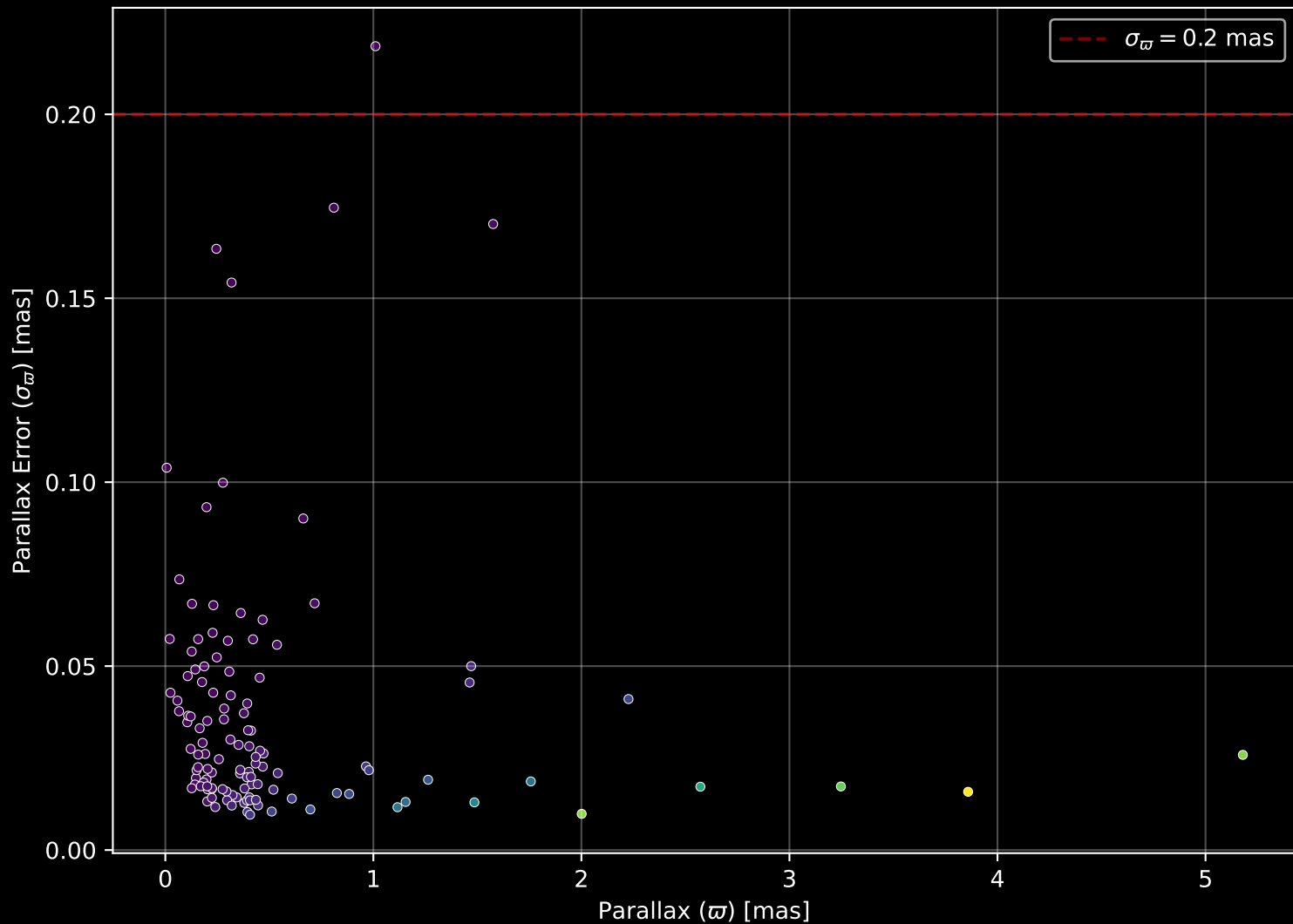
APOGEE DR17 Field: [288-00-C] Parallax Quality (n= 119)
