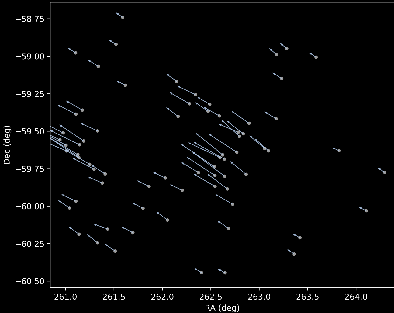
APOGEE DR17 Cluster 1 Proper Motion Vectors (n=70)
